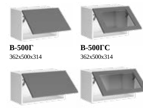
В-500Г 362x500x314 В-500ГС 362x500x314 В-600Г 362x600x314 В-600ГС 362x600x314
