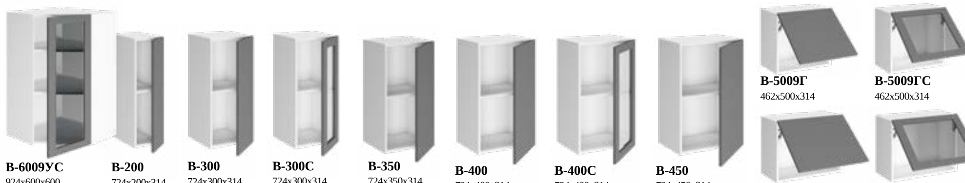
В-6009УС 924x600x600 В-200 724x200x314 В-300 724x300x314 В-300С 724x300x314 В-350 724x350x314 В-400 724x400x314 В-400С 724x400x314 В-450 724x450x314 В-5009Г 462x500x314 В-5009ГС 462x500x314 В-6009Г 462x600x314 В-6009ГС 462x600x314
